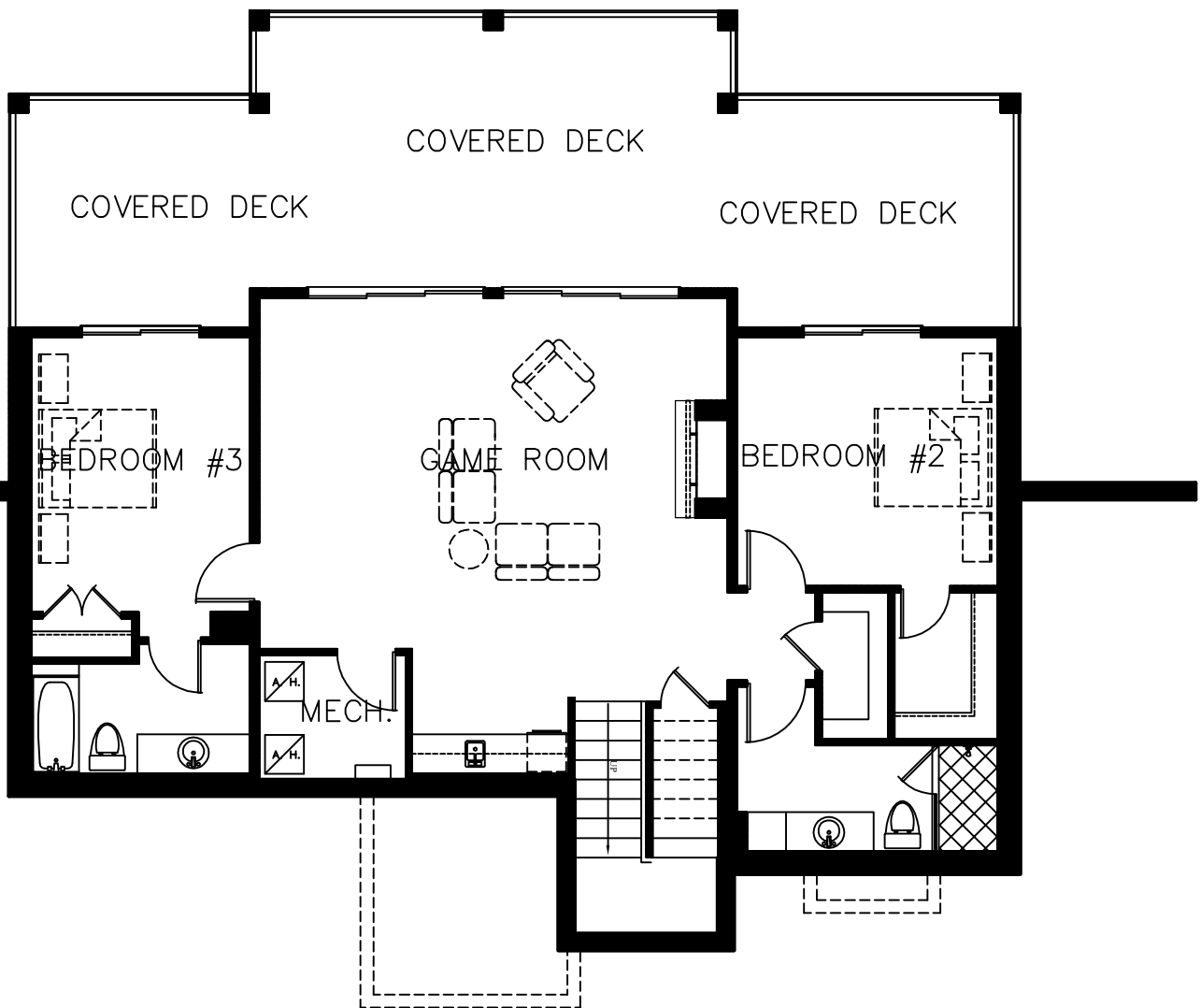
LOWER FLOOR LAYOUT SCALE: 1/4" = 1'-0"
